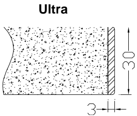
Square edge detail for veneered tables, 30mm with 3mm wooden lip.
